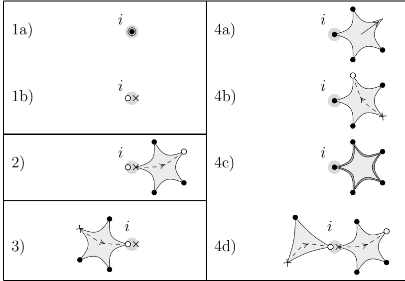
Figure 2: Possible ways of saturating the Grassmann fields on vertex i (indicated by the small gray disk).
