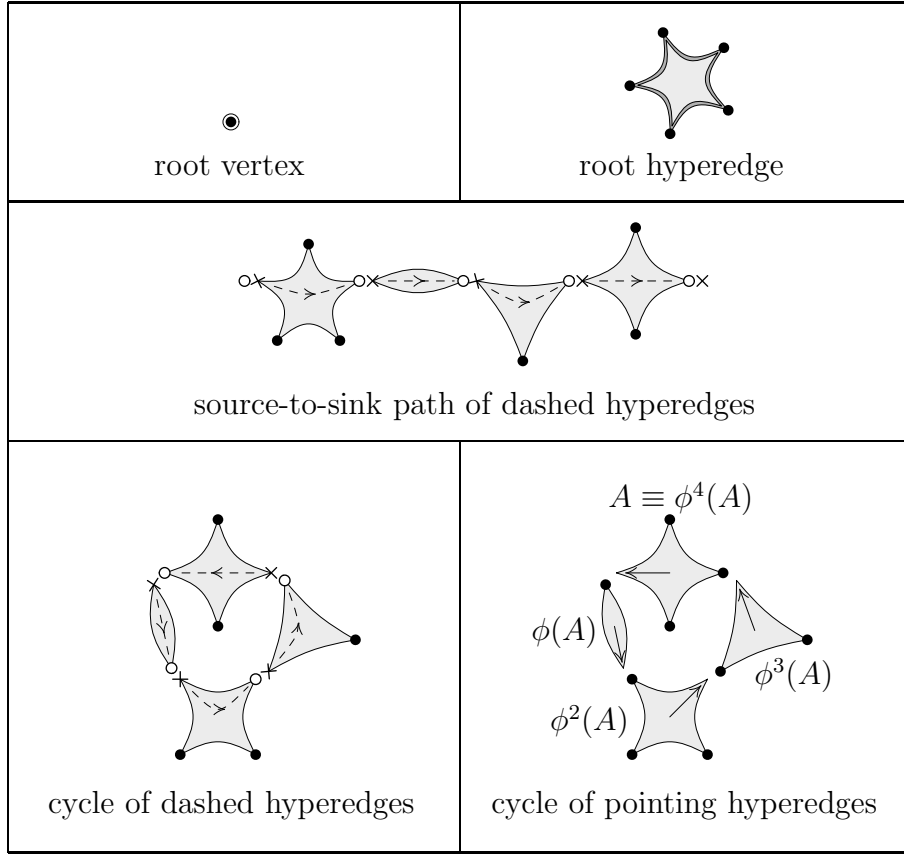
Figure 3: The five kinds of root structures.
